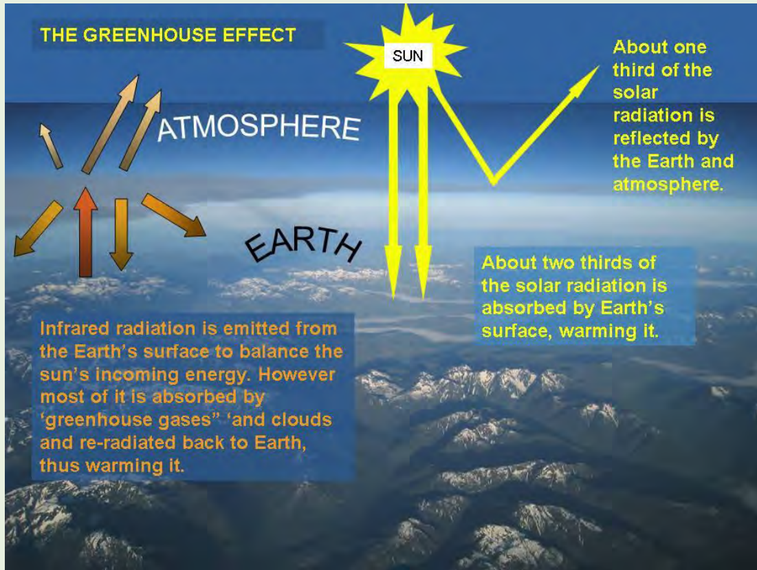
Figure 1. Diagram to illustrate the natural 'Greenhouse Effect'.
